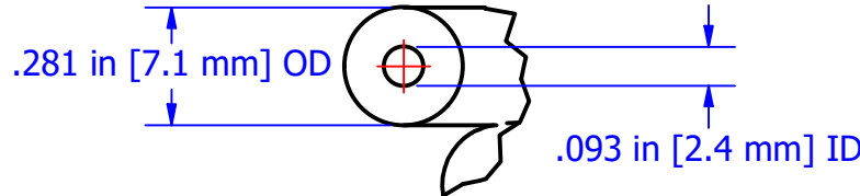
DETAIL A SCALE 2 : 1
